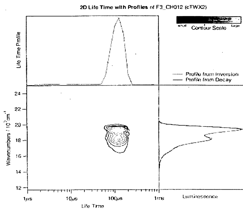
FIGURE 3 (I) in Cyclohexane at 80K
